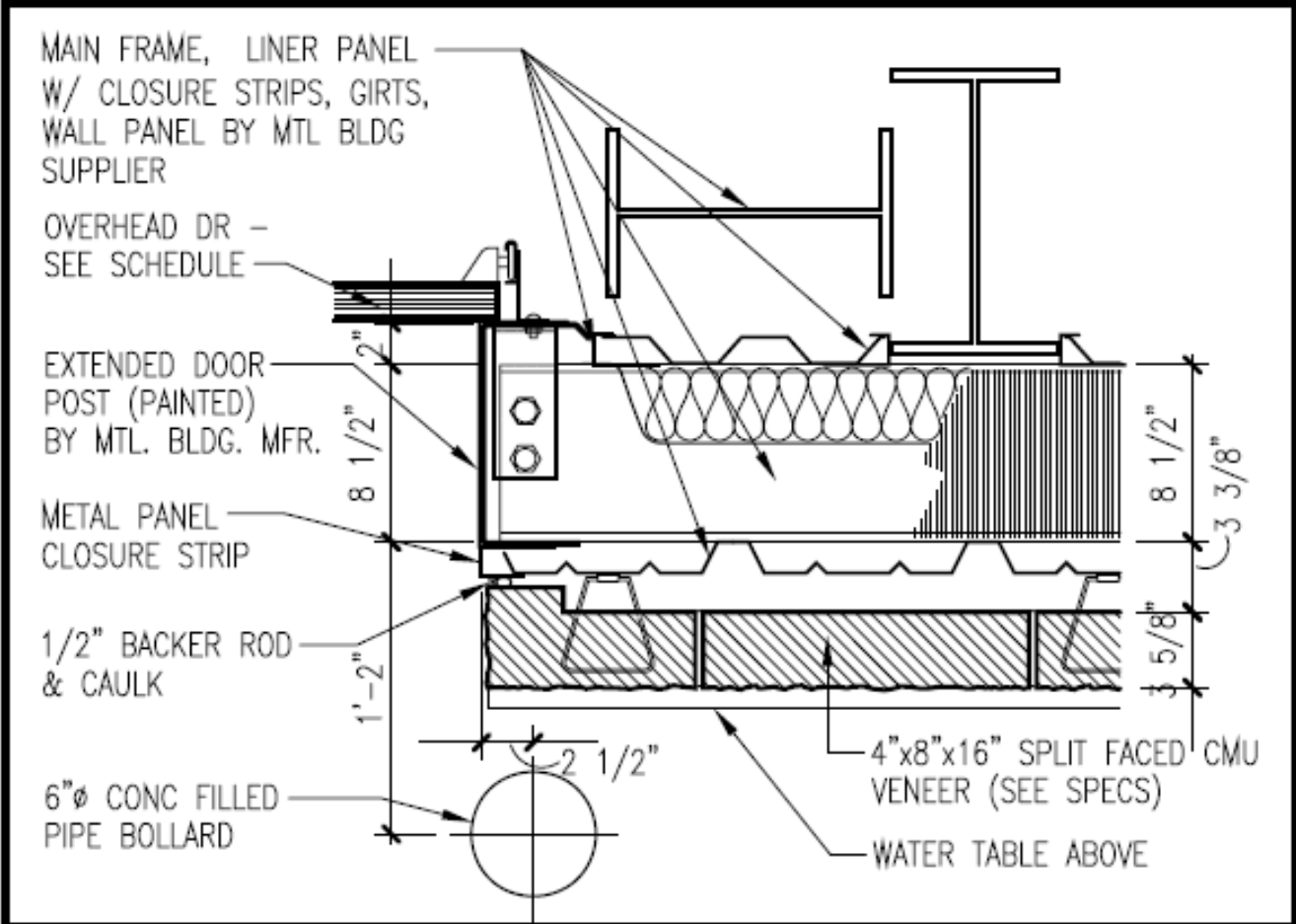
21 JAMB DETAIL 1"=1'-0" AT OVERHEAD DOOR AND MASONRY WAINSCOT
