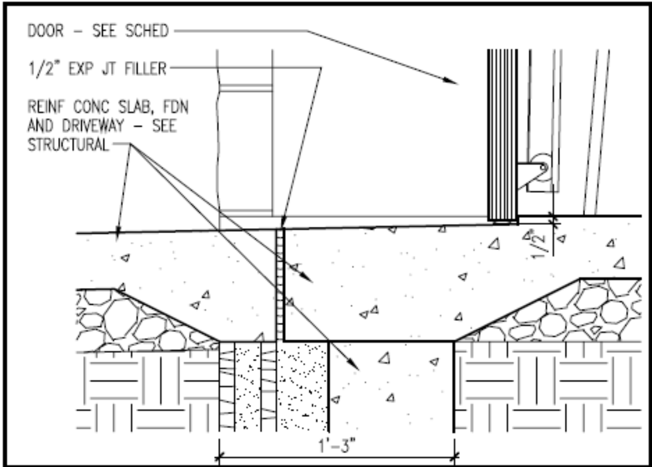
19 THRESHOLD DETAIL 1 1/2"=1'-0" AT OVERHEAD DOOR
