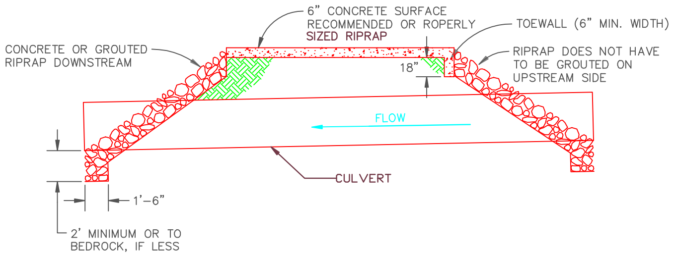
CROSS-SECTION
