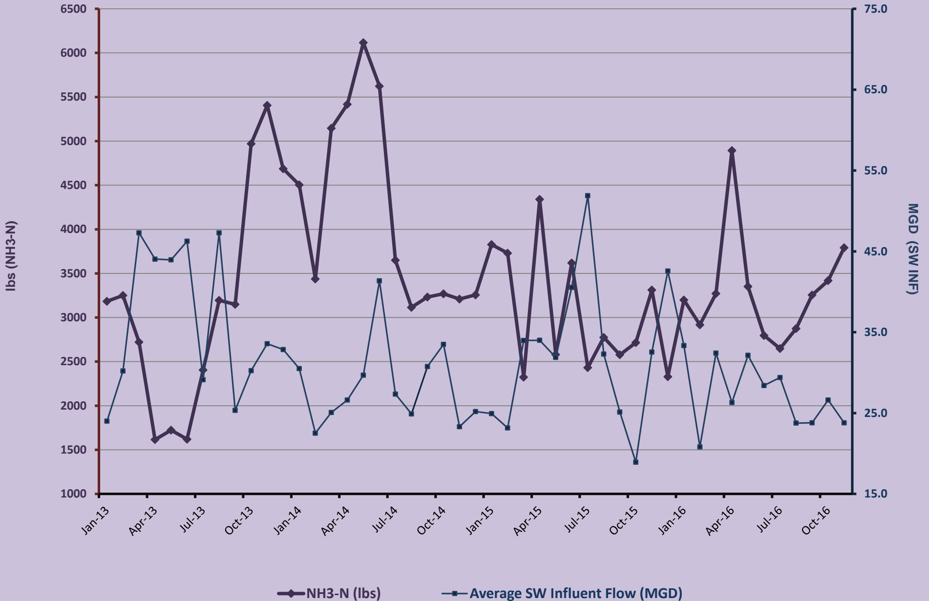
SW Influent Ammonia (lbs) with SW Influent Flow (MGD) January 2013 - November 2016 Monthly Average
